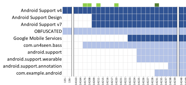
Figure 2: Libraries included in Smart Audiobook Player
