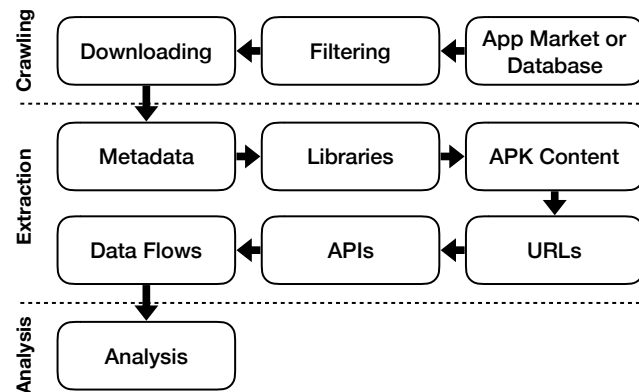
Figure 1: Main components and analysis flow of Cartographer
