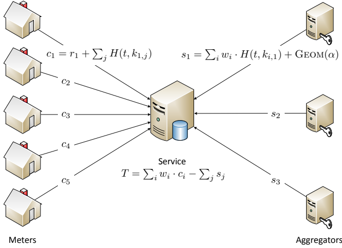
Fig. 4. Aggregation of readings using weights \vec{w} in an infrastructure with 5 meters and 3 aggregators. The setup phase ensures that meter i and aggregator j share a key k_{i,j} .
